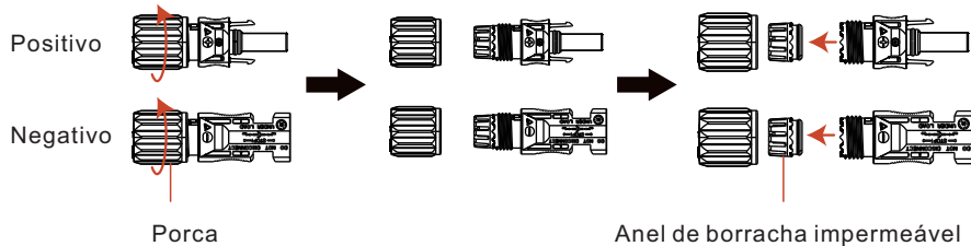
Figura 5.11 Remova a tampa do conector do terminal
